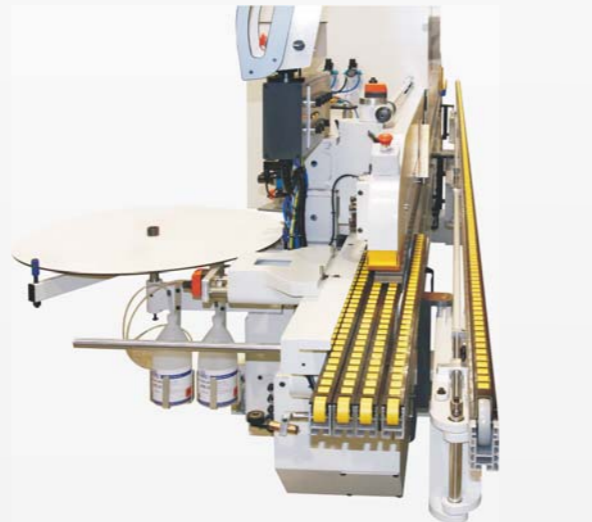
26.1.5 meter outboard support roller rail 1.5米舷外支撐滾輪架,多連桿機構確保平行移動
