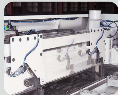
Independent side press roller system, automatic align the cross cutting at right angle.
