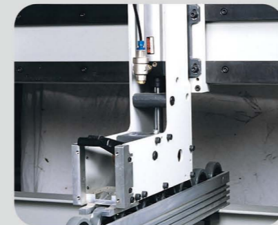
Extra size floating gripper with close-loop clamping force sensor.
